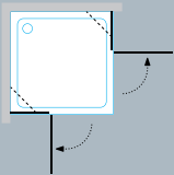
Q 100, 90, 80 100x100 / 90x90 / 80x80
